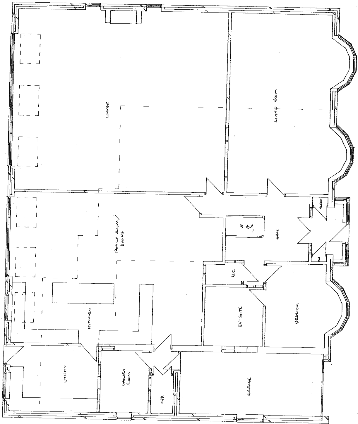
PROPOSED GROUND FLOOR 1:100
